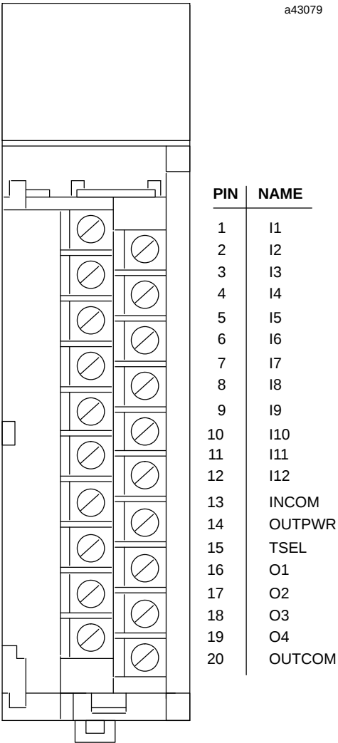
Figure 2-4. Terminal Board Pin Assignments
