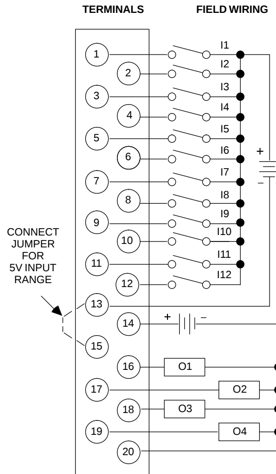
Figure 2-5. Field Wiring for the High Speed Counter
