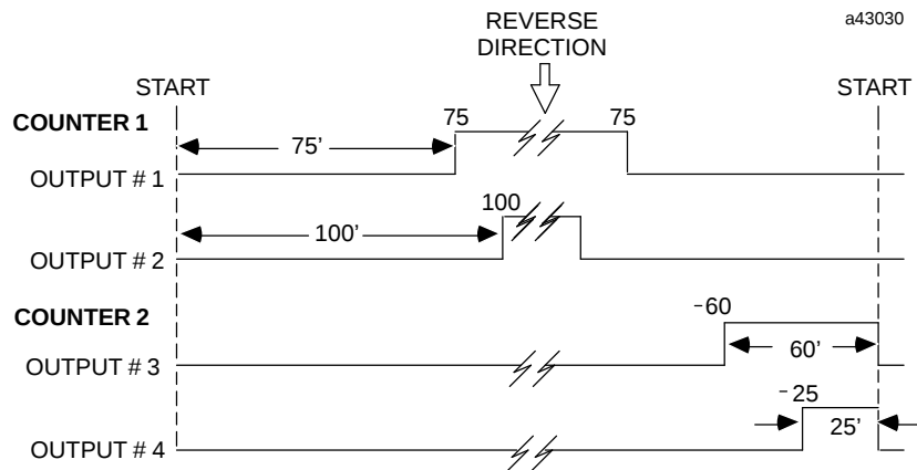
Figure A-2. Output Timing Conditions Example
