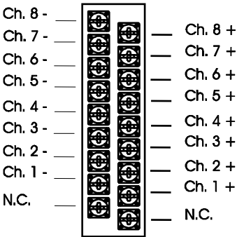
Figure 3 – Terminal Block With Block Terminal
