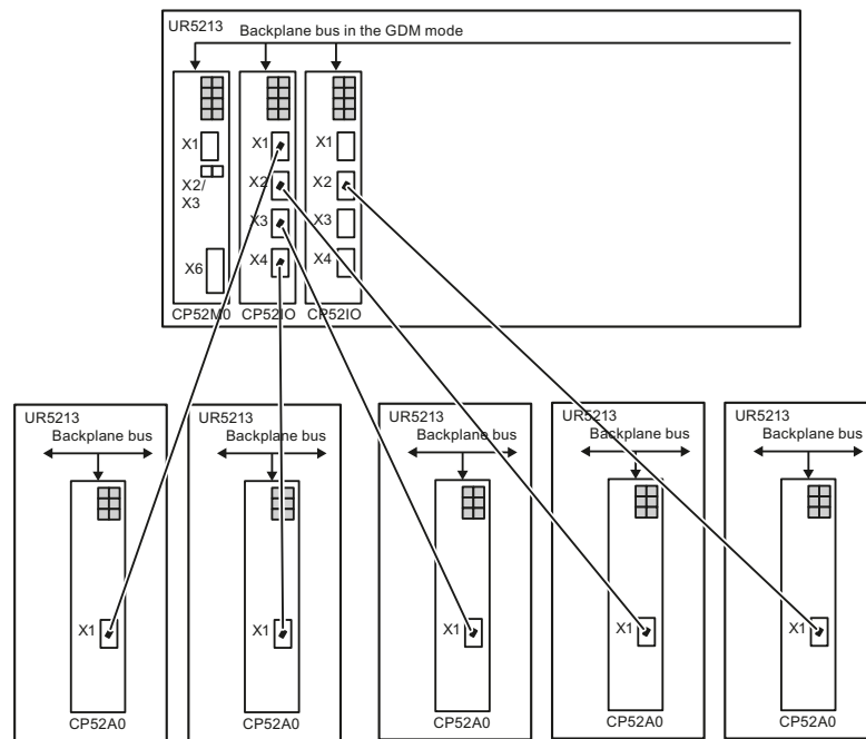
Figure 7-9 Example of a GDM system with 5 racks that are coupled with FOCs
