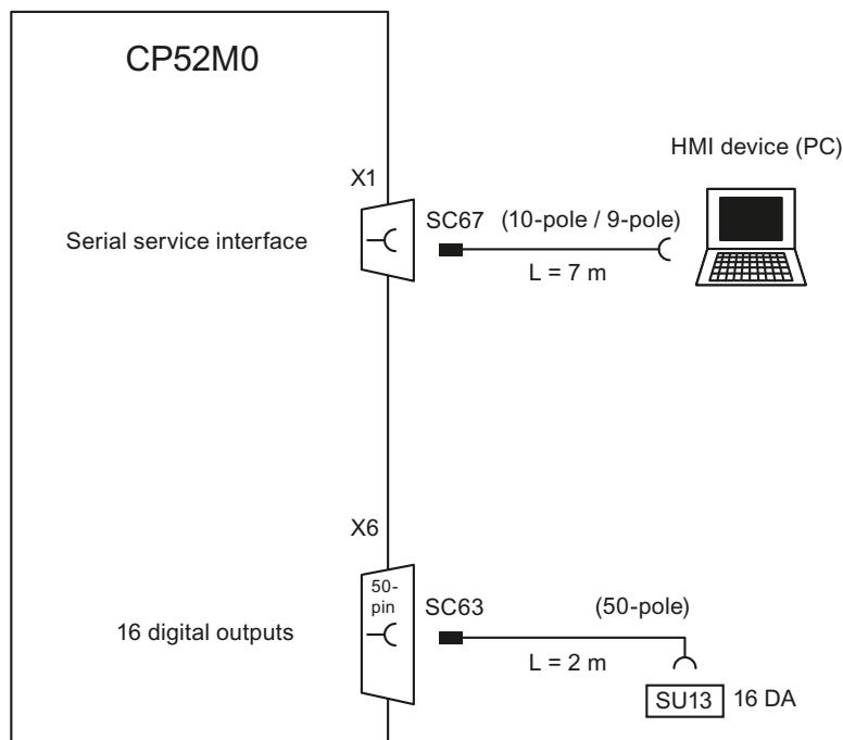
Figure 7-8 Connection options of CP52M0
