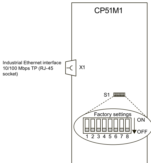
Figure 7-4 Connection options of CP51M1
