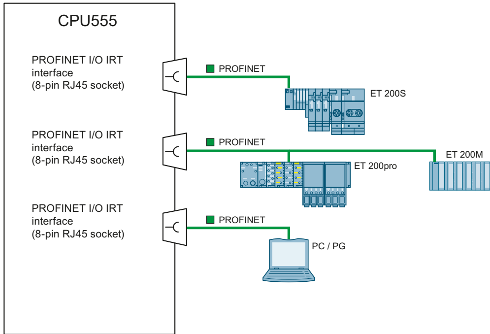
Figure 5-2 Connection examples of CPU555
