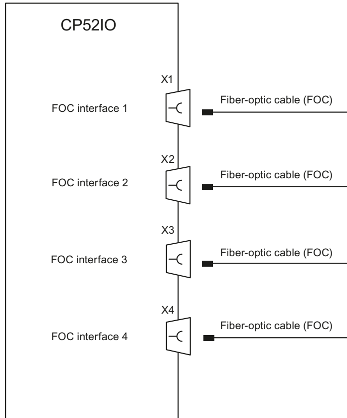
Figure 7-11 Connection options of CP52IO
