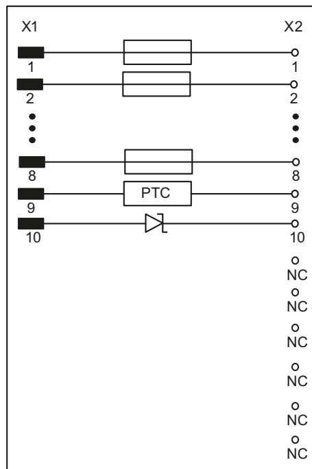
Figure 8-13 SU12 circuit diagram
