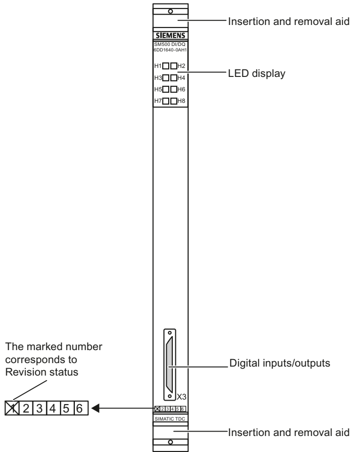
Figure 6-3 Front panel of SM500 DI/DQ
