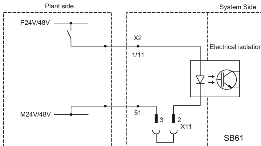
Figure 8-5 Position of the jumpers for electrically isolated inputs
