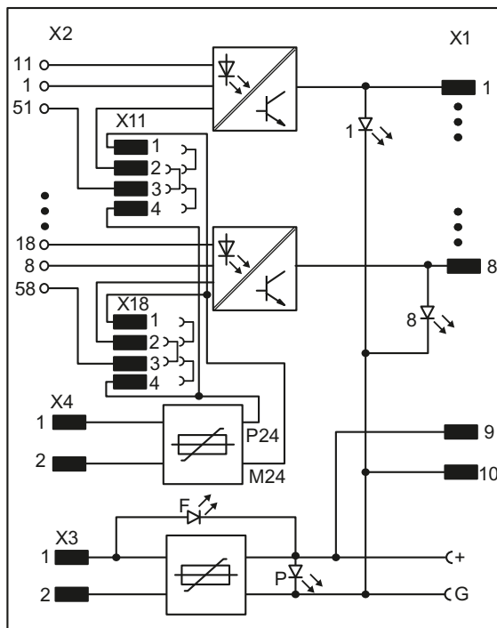
Figure 8-8 Block diagram of interface module SB61
