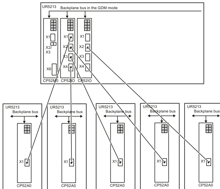
Figure 7-5 Example of a GDM system with 5 racks that are coupled with FOCs
