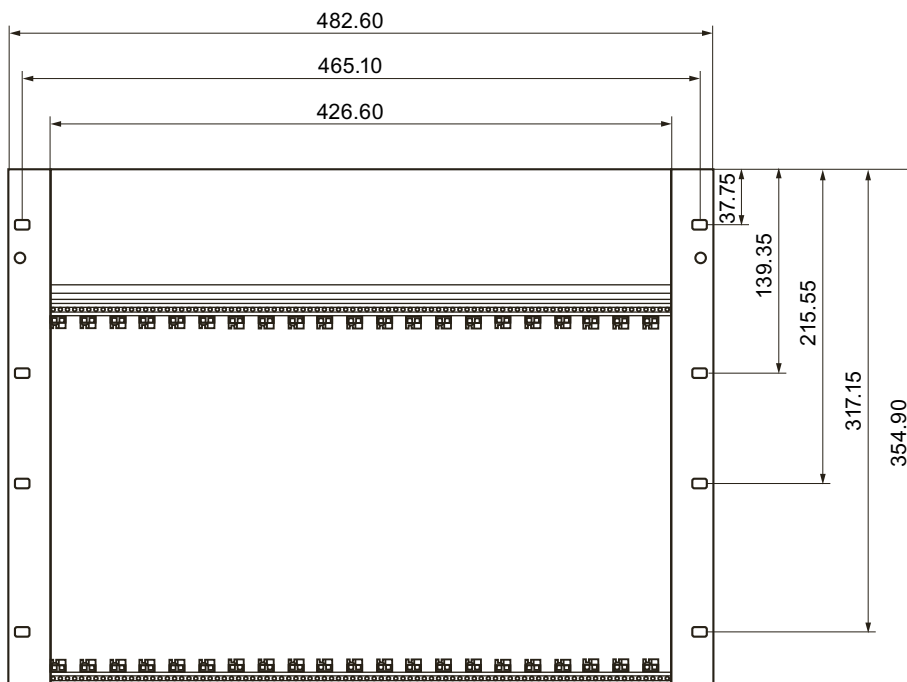
Figure 4-6 Dimensional drawing of rack UR5213
