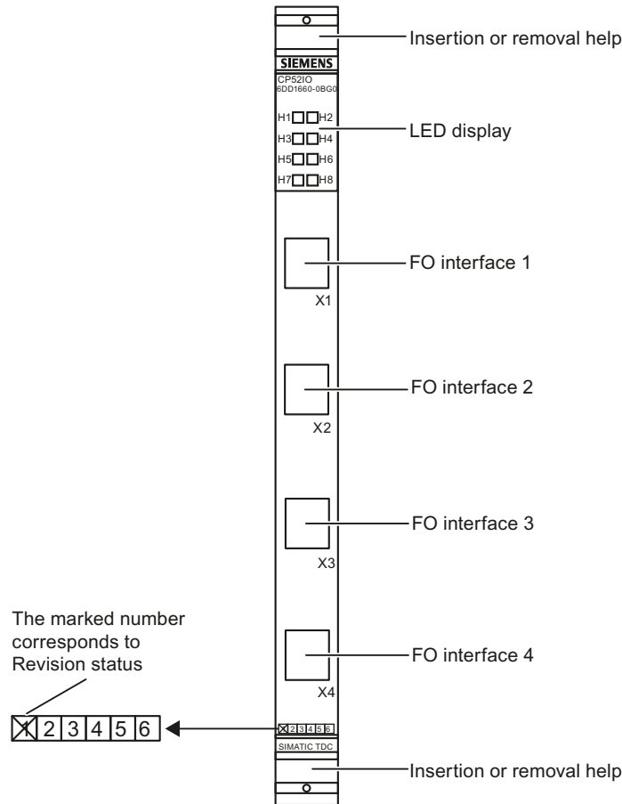
Figure 7-10 Front panel of CP52IO
