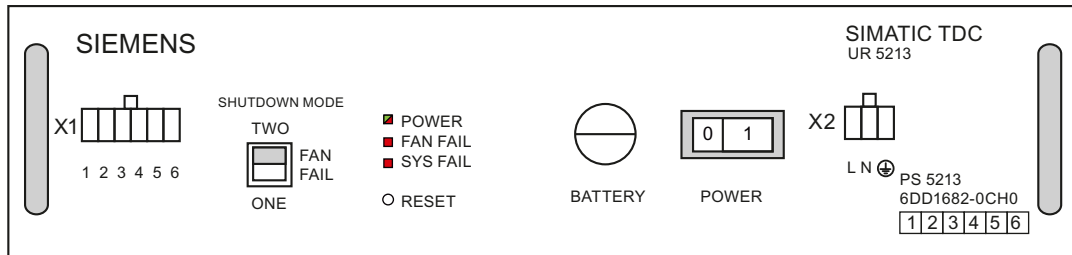
Figure 4-8 Front view of the power supply unit
