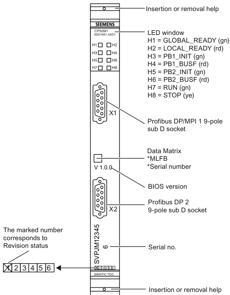
Figure 7-1 Front panel of CP50M1
