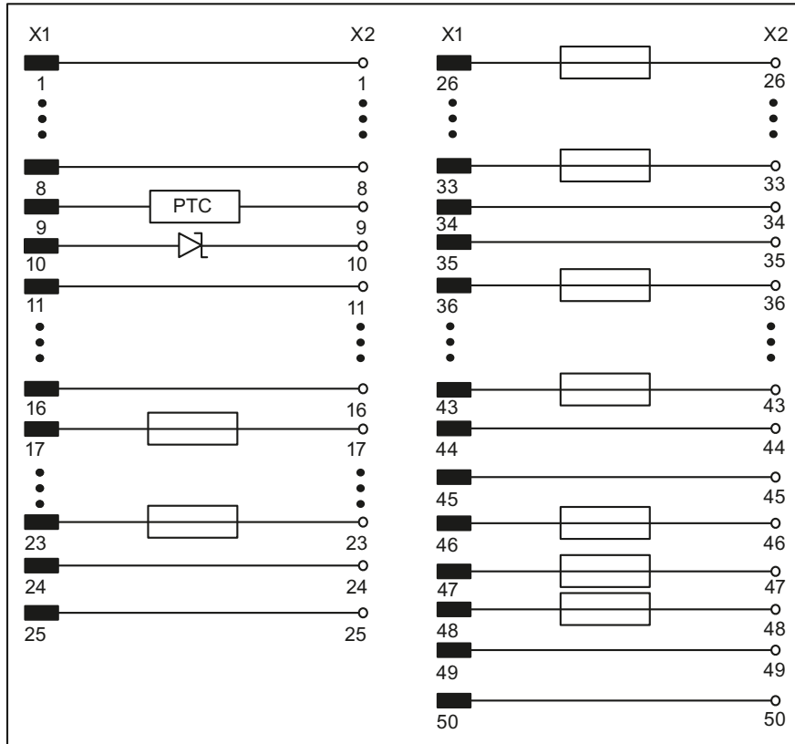
Figure 8-14 SU13 circuit diagram
