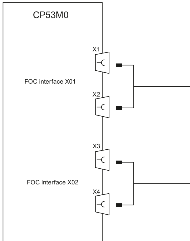
Figure 7-19 Connection options of CP53M0
