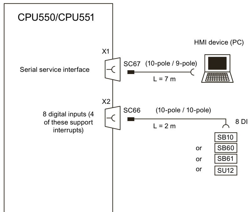
Figure 5-4 Connection options of CPU550/CPU551
