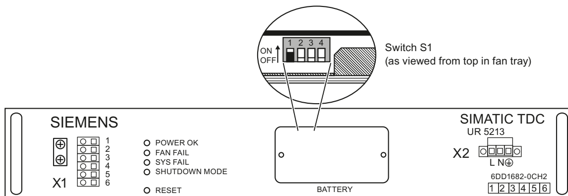
Figure 4-5 Front view of the fan tray
