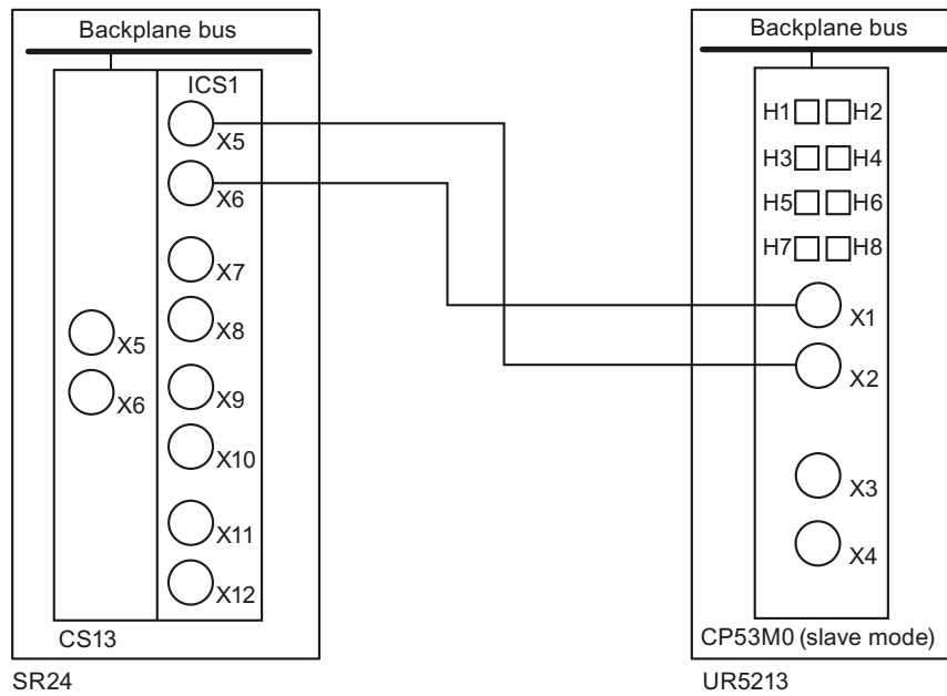
Figure 7-15 Options for connecting CP53M0 as slave to the CS13
