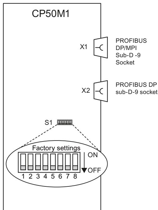
Figure 7-2 Connection options of CP50M1
