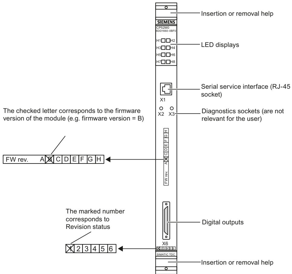
Figure 7-6 Front panel of CP52M0
