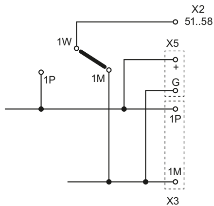
Figure 8-1 Soldering bridge for setting the signal reference points
