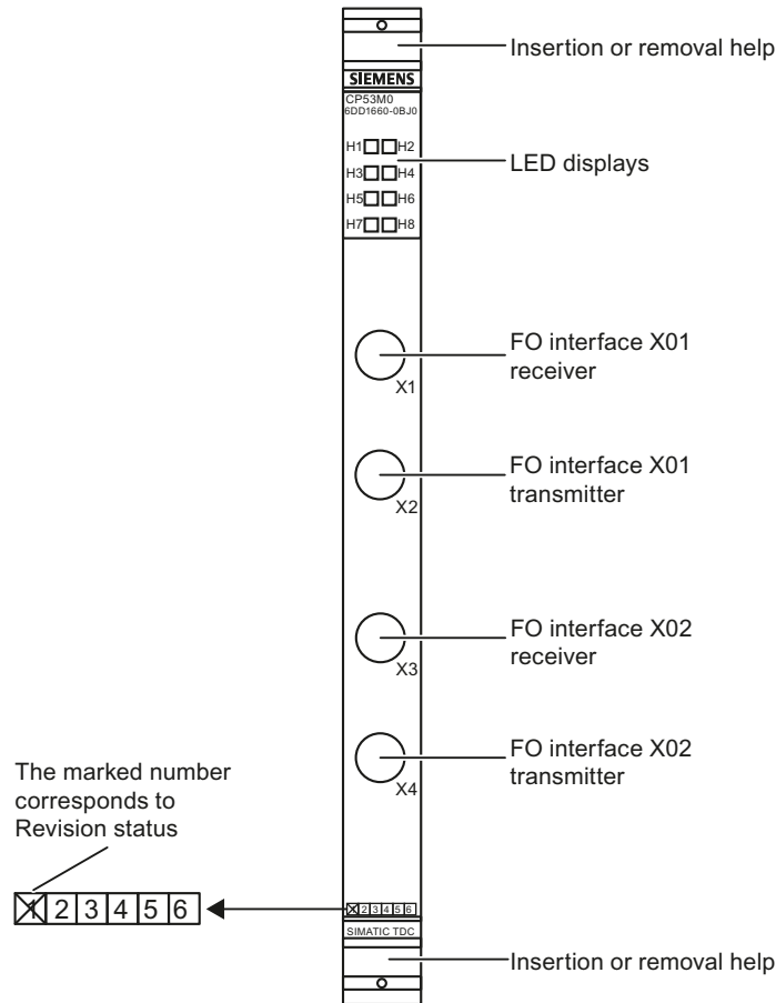
Figure 7-18 Front panel of CP53M0
