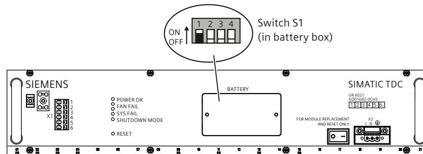
Figure 4-2 Front view of the fan tray
