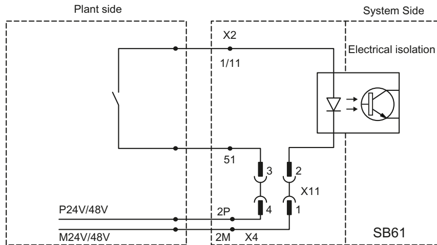
Figure 8-6 Position of the jumpers for inputs with common reference potential
