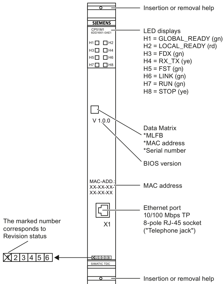
Figure 7-3 Front panel of CP51M1
