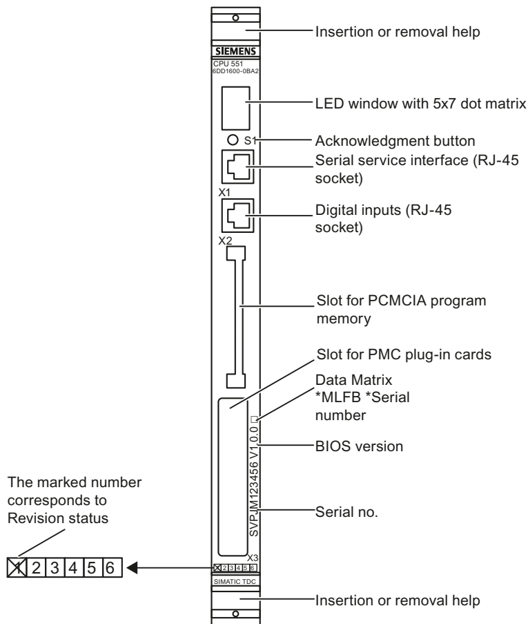
Figure 5-3 Front panel of CPU551
