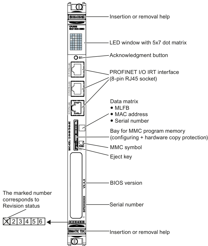
Figure 5-1 Front view of CPU555
