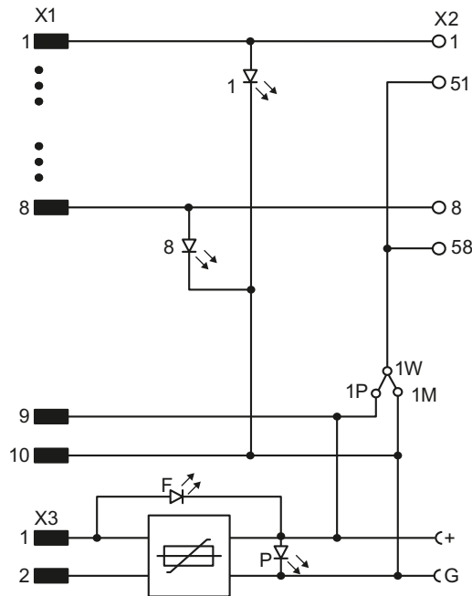
Figure 8-3 Block diagram of interface module SB10
