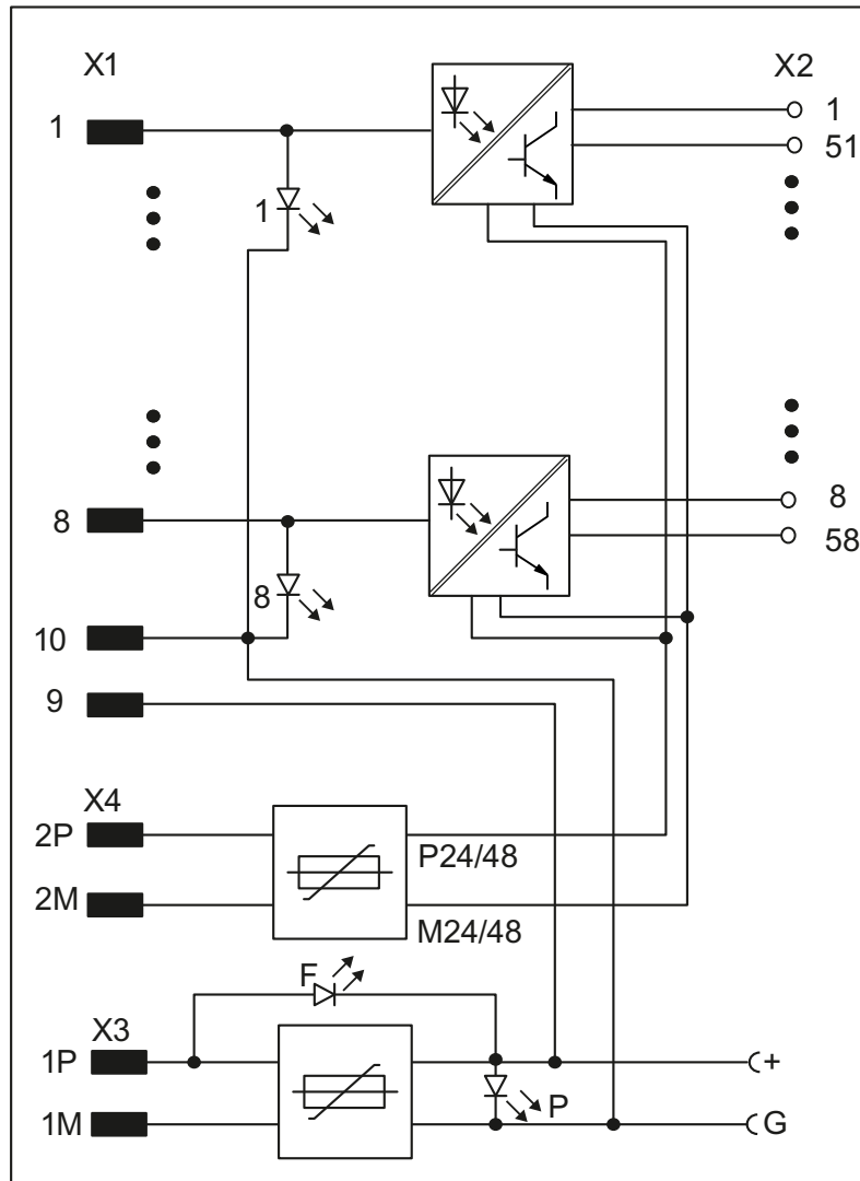
Figure 8-12 Block diagram of interface module SB71
