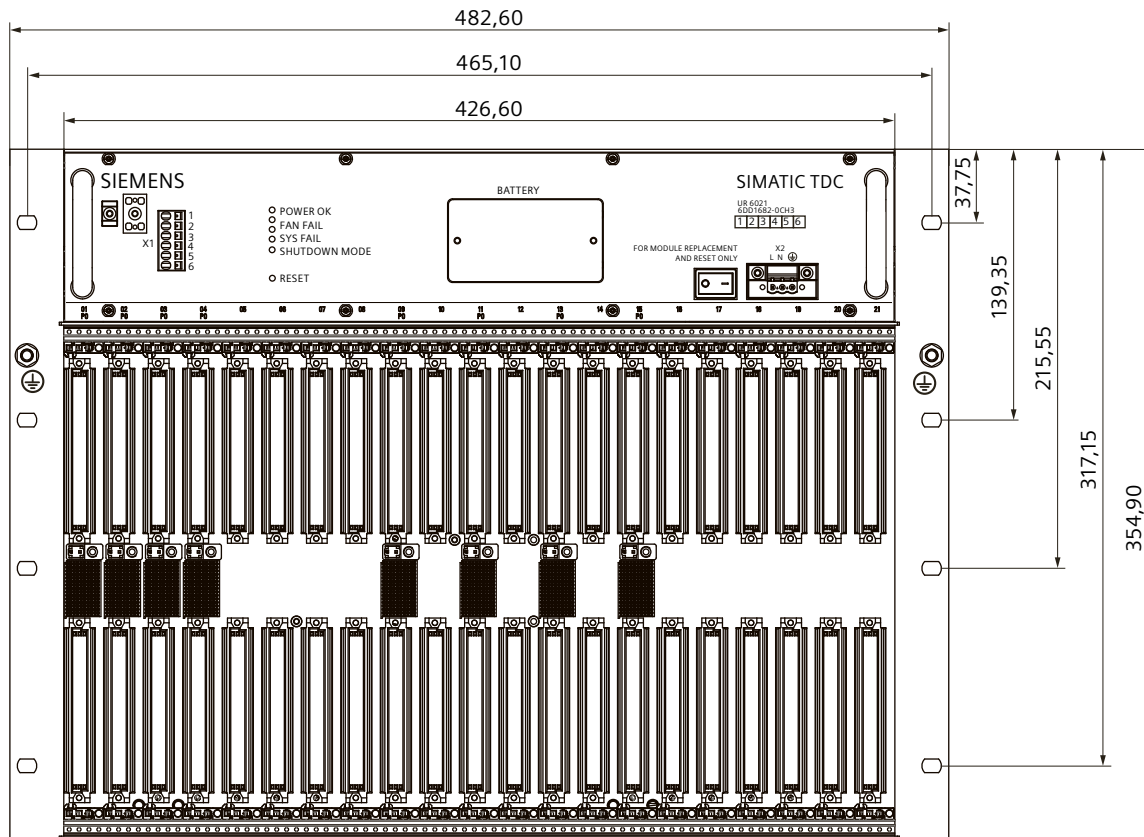
Figure 4-3 Dimension drawing of rack UR6021
