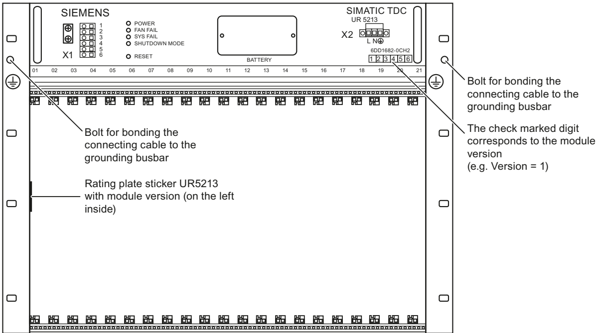
Figure 4-4 Rack UR5213 (front view)
