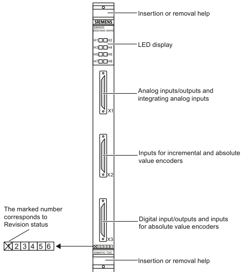
Figure 6-1 Front panel of SM500
