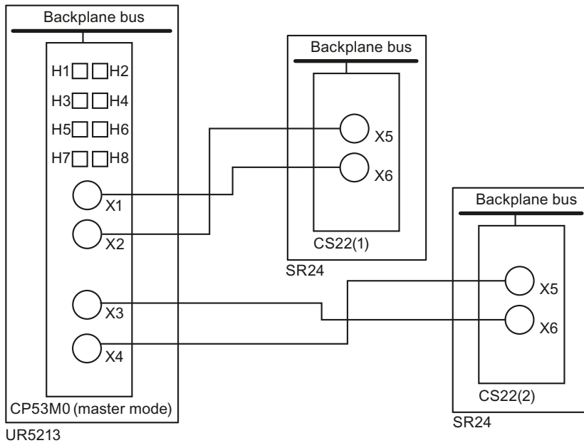
Figure 7-16 Options for connecting the CS22 to CP53M0 that is operating in master mode
