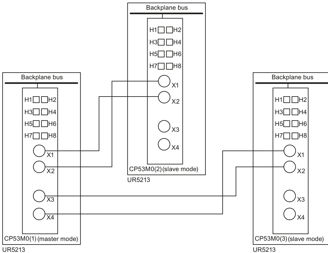
Figure 7-17 Coupling three SIMATIC TDC racks
