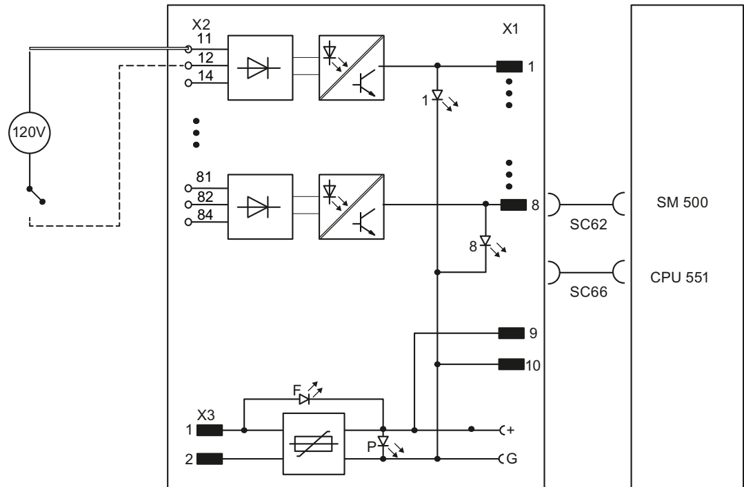
Figure 8-4 Block diagram of interface module SB60
