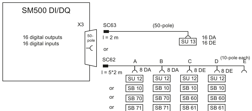
Figure 6-4 Connection options for the SM500 DI/DQ
