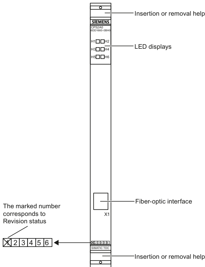
Figure 7-13 Front panel of CP52A0
