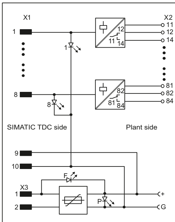
Figure 8-10 Block diagram of interface module SB70
