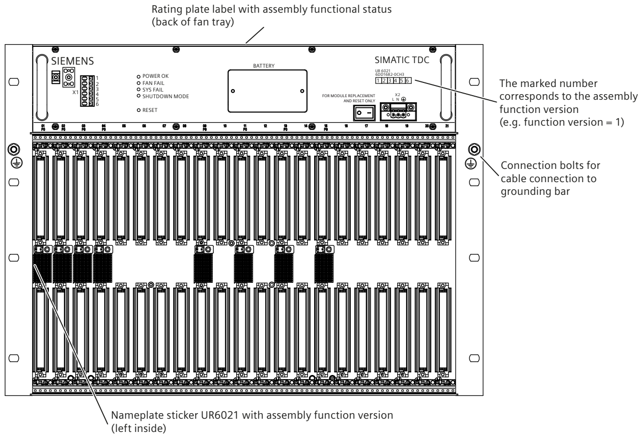
Figure 4-1 Rack UR6021 (front view)
