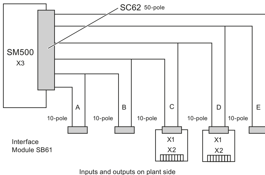
Figure 8-7 Application example of an SB61 interface module on digital I/O module SM500
