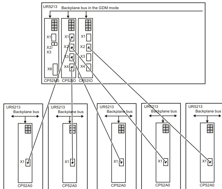
Figure 7-12 Example of a GDM system with 5 racks that are coupled with FOCs
