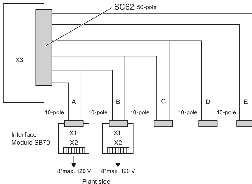
Figure 8-9 Application example of an SB70 interface module on digital I/O module SM500
