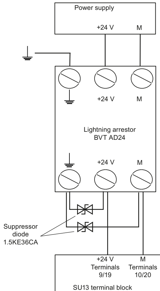
Figure 7-7 Circuit for the suppressor diodes on the lightning arrester
