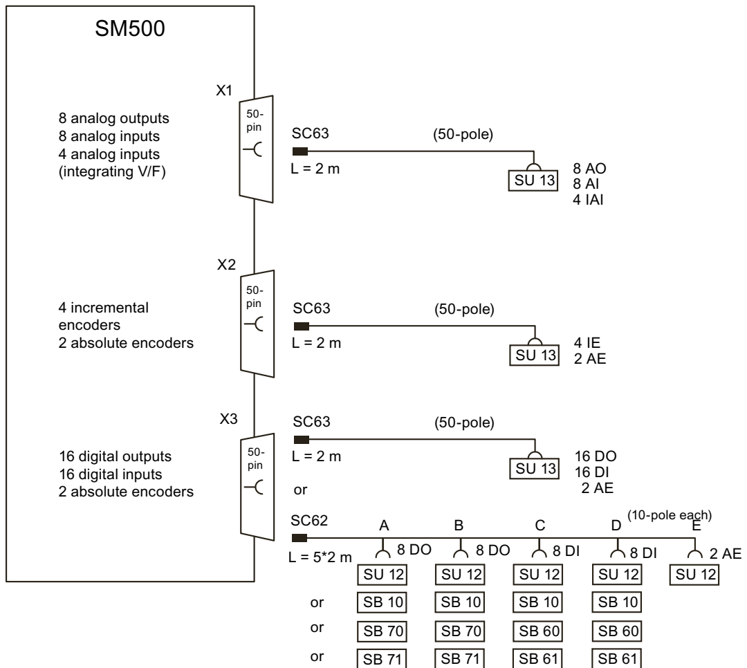
Figure 6-2 Connection options of SM500
