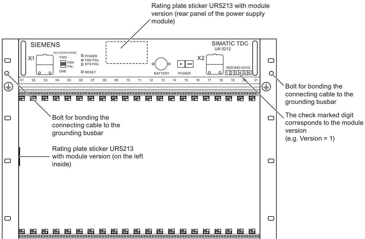
Figure 4-7 Rack UR5213 (front view)
