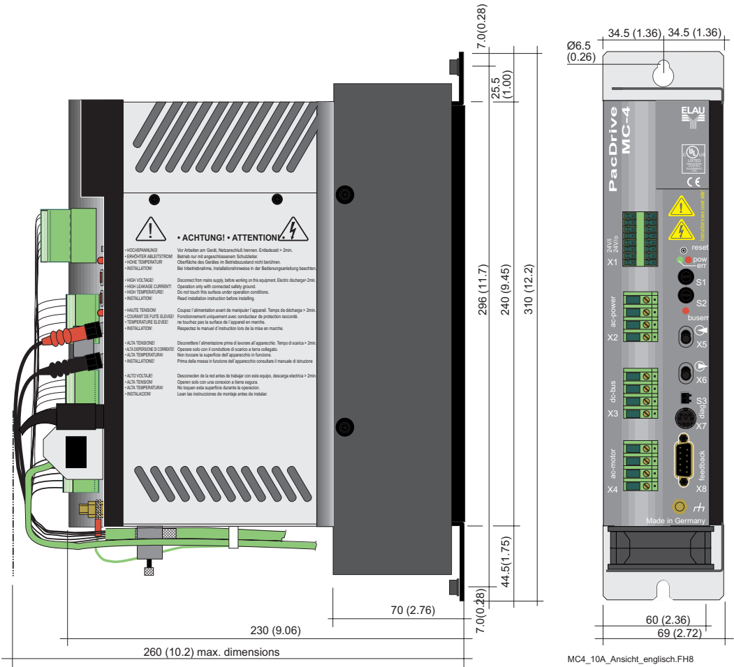
Fig. 4-3: Dimensions of the MC-4 / 10 A
