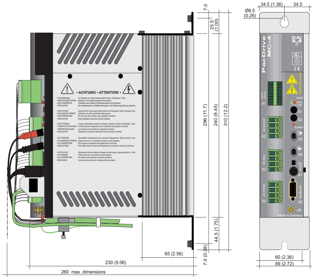
Fig. 4-1: Dimensions of the MC-4 / 1.5 A and 3 A
