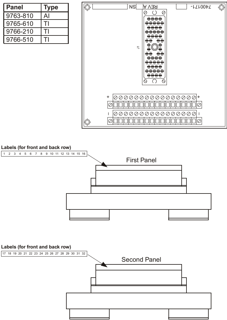
Figure 270 16-Point Non-Commoned AI/TI Panel Label Placement
