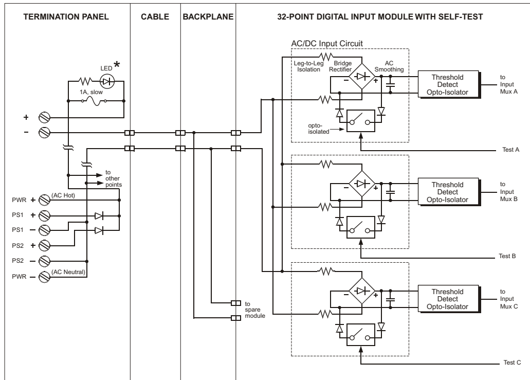
Figure 9 Simplified Schematic of a 3503E or 3505E DI Module with a 9563-810 Panel
