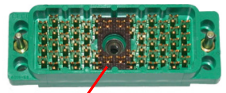
installed gasket
