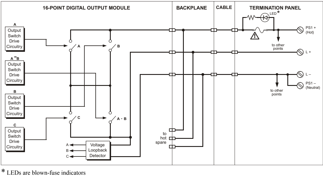
Figure 68 Simplified Schematic of a 3601E DO Module with a Commoned DO Panel
