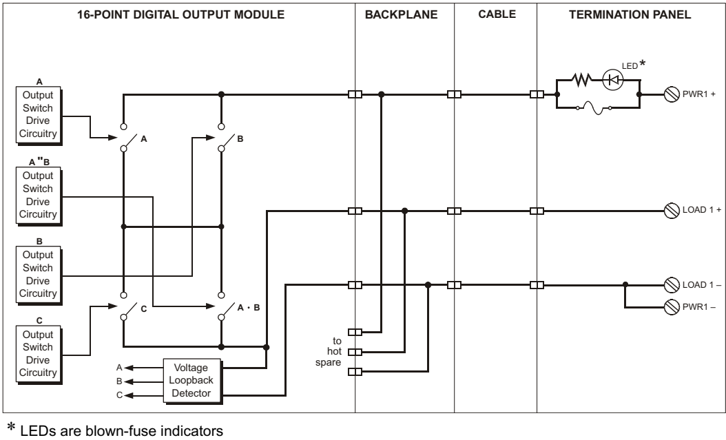
Figure 99 Simplified Schematic of a 3601E or 3601T DO Module with a Non-Commoned DO Panel
