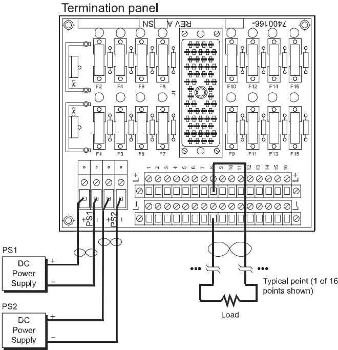
Figure 78 Field Wiring for 9662-810 with a 3604E Module
