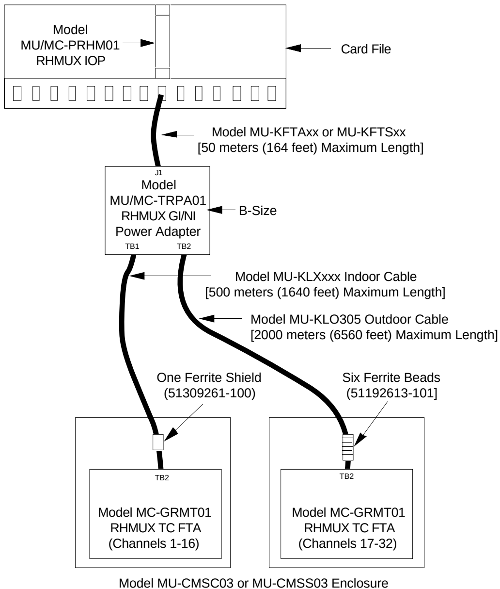
Figure 12-3 Nonincendive RHMUX Configuration Interconnections
