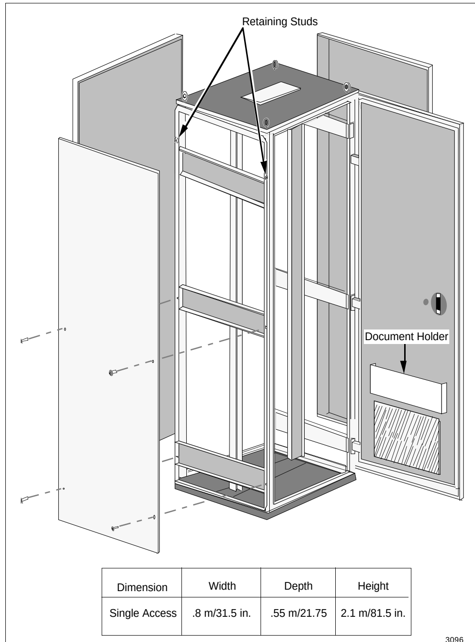
Figure 8-1 Single-Access Cabinet
